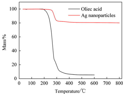
Fig. 5. TGA curves of oleic acid and Ag nanoparticles.
